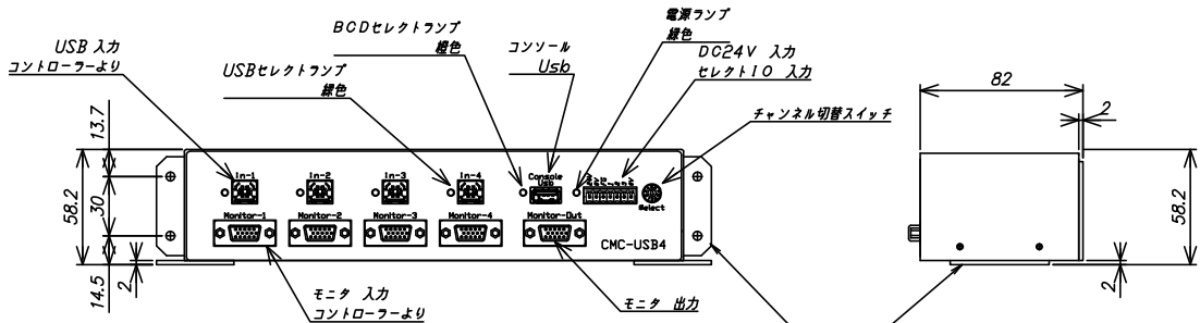
4Ch CMC-USB4
