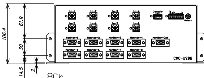
8Ch CMC-USB8
